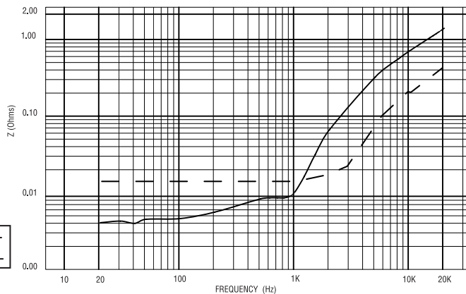
Figure 1 CH1, CH2, and CH4 Output Impedance
